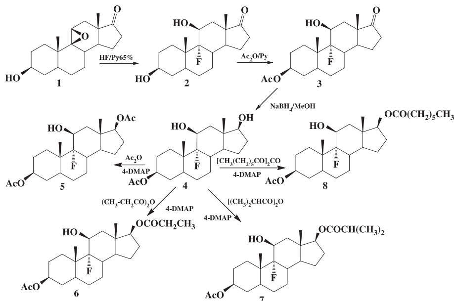
Scheme 1. Synthesis of fluorosteroid derivatives and their esters.
